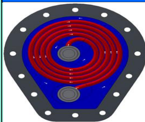
Figure 1. Spiral Flow Path
